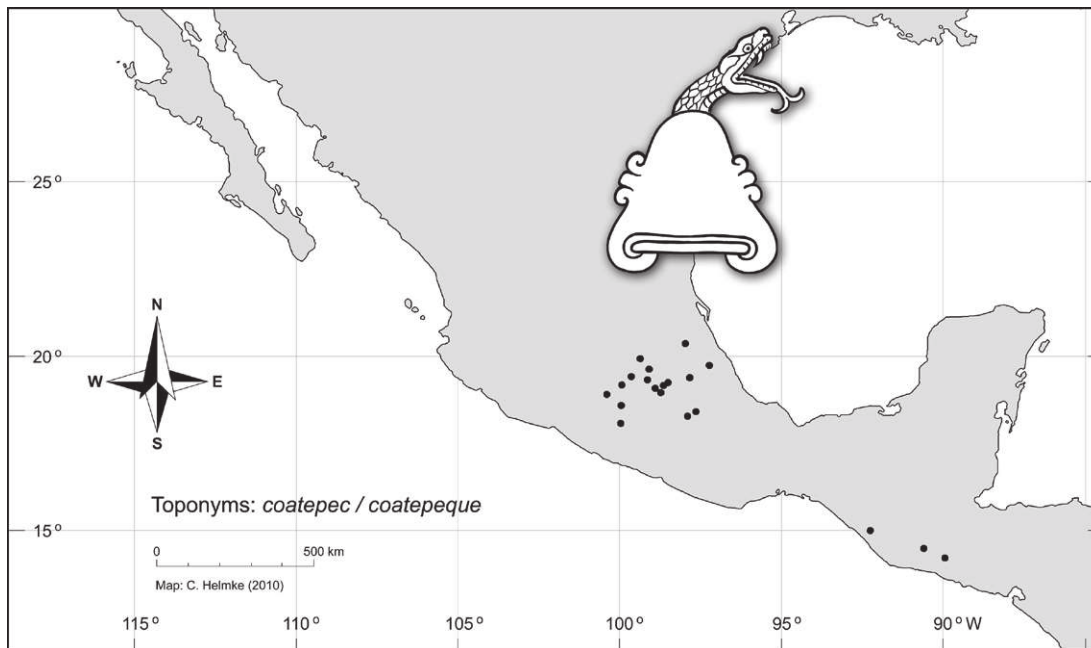
Fig. 15. Map of Mesoamerica showing the distribution of toponyms named Kōwātepēk <Coatepec ~ Coatepeque>. Note the concentration of place names in central Mexico and the outliers on the Pacific coast of Guatemala (map by Christophe Helmke).
